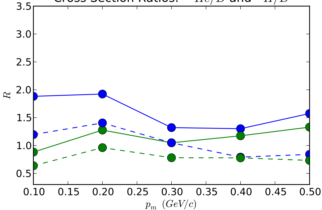
Cross Section Ratios: {}^3\text{He}/D and {}^3\text{H}/D
