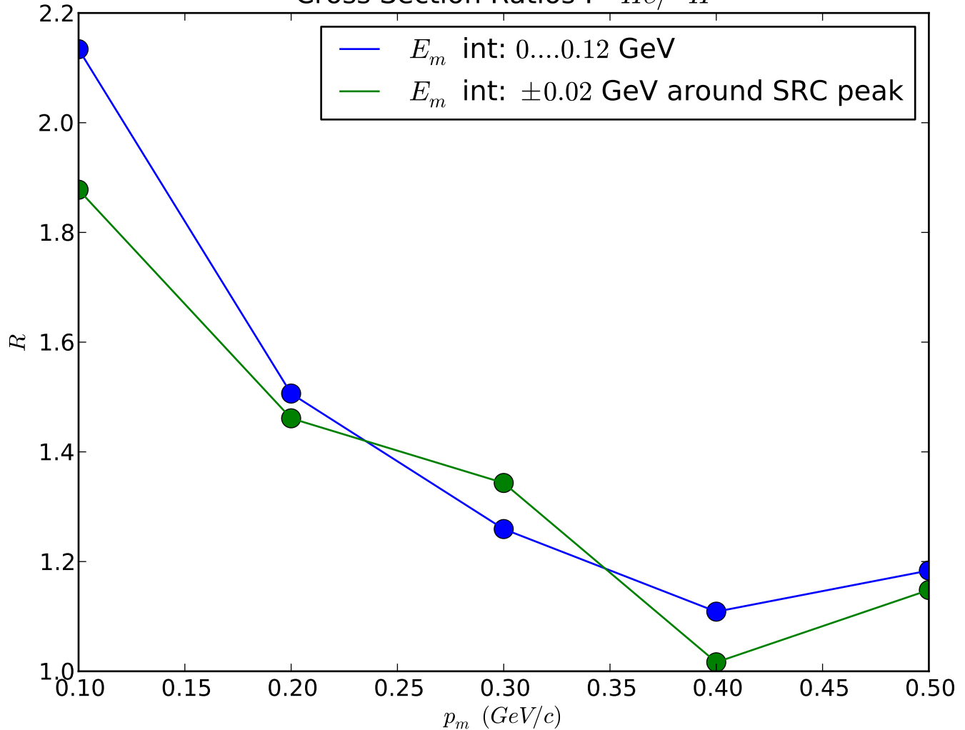
Cross Section Ratios : {}^3\text{He}/{}^3\text{H}
